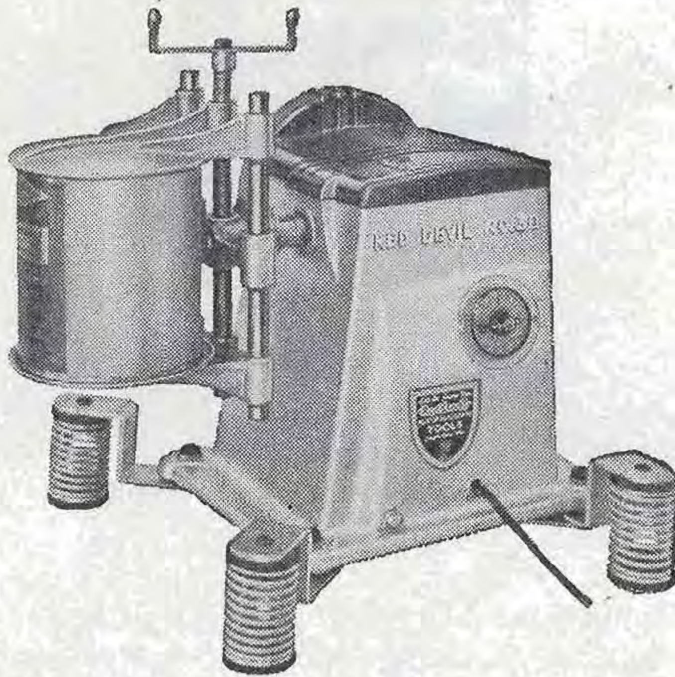
Cut shows conditioner mounted on spring counter base.
