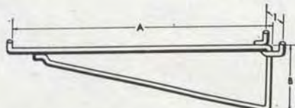
No. C188—A 7\frac{13}{16} in. B 2\frac{1}{4} in.
