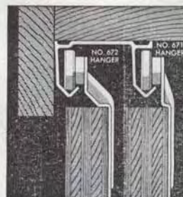
\frac{5}{8} to \frac{3}{4} Inch Door Thickness 672 on Front—671 on Rear
