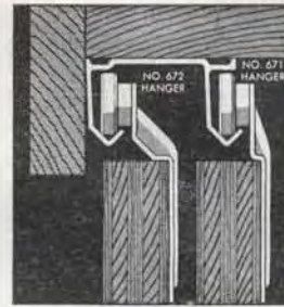
5/8 to 3/4 Inch Door Thickness 672 on Front—671 on Rear
