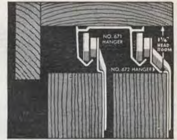
1 to 1 3/8 Inch Door Thickness 671 on Front—672 on Rear
